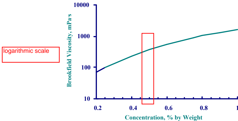
Figure 4: Viscosity vs. Concentration of VANZAN NF
