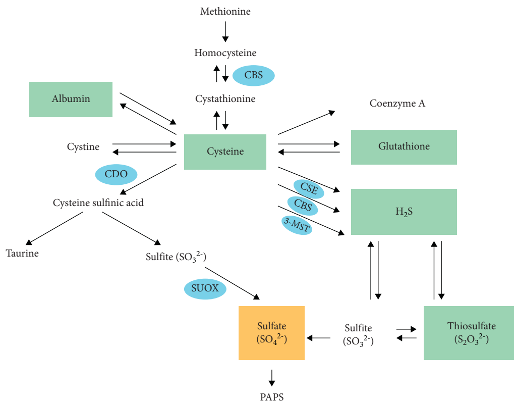
FIGURE 2: Sulfur metabolism diagram. The essential sulfur amino acid methionine converts to cysteine, a precursor to albumin, cystine, coenzyme A, glutathione, hydrogen sulfite ( H_2S ), taurine, and sulfate ( SO_4^{2-} ). H_2S can convert to thiosulfate ( S_2O_3^{2-} ) and sulfite ( SO_3^{2-} ), which are oxidised to sulfate. The enzyme cystathionine- \beta -synthase (CBS) converts homocysteine to cystathionine, while cysteine dioxygenase (CDO) is responsible for the conversion of cysteine to cysteine sulfinic acid. Sulfite oxidase (SUOX) oxidises sulfite to sulfate. H_2S is generated from cysteine by three different pathways through either CBS, cystathionine- \gamma -lyase (CSE), or 3-mercaptopyruvate sulfurtransferase (3-MST). Adapted with permission by CC by 4.0 [3].
