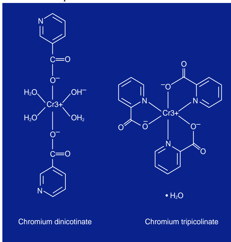
Figure 2. Structure of Chromium Dinicotinate and Chromium Tripicolinate
