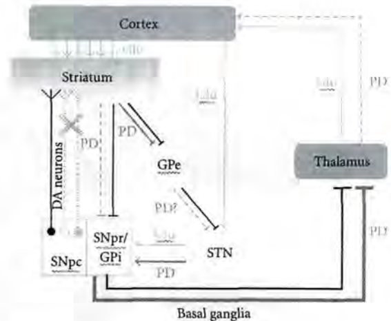
FIGURE 1: Basal ganglia motor circuit in Parkinson's disease: dopaminergic neurons (DA) create a direct pathway between Substantia Nigra pars compacta (SNpc) and striatum—the input nuclei of the basal ganglia. Another direct pathway connects the striatum to the internal segment of globus pallidus (GPi) and the substantia nigra pars reticulata (SNpr). GPi and SNpr are the output nuclei of the basal ganglia, which projects to the thalamus and from there to the cortex. The indirect pathway connects the striatum to output nuclei through external segment of the globus pallidus (GPe) and then subthalamic nucleus (STN). In Parkinson's disease (PD), the dopaminergic input from SNpc is progressively lost, causing a reduction in the direct pathway signal. Indirect pathway increases its activity through STN in the output nuclei and has inhibitory influence on the thalamus. It leads to a reduction of thalamic glutamatergic input on the motor cortex and subsequent reduction in movement, as rigidity and bradykinesia are observed in PD patients.
