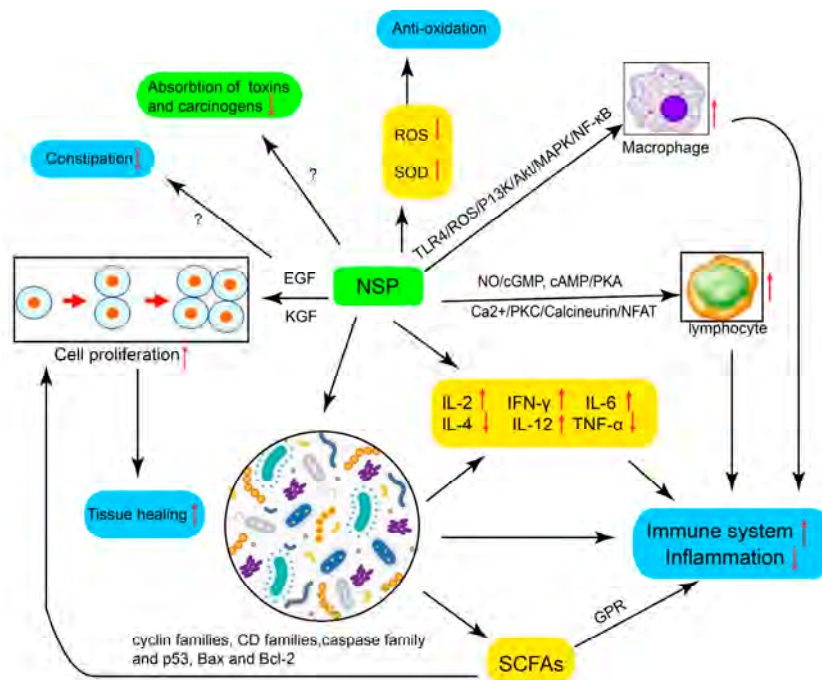
Figure 3. The possible molecular mechanisms of NSPs affecting IBD. NSP: non-starch polysaccharide; ROS: reactive oxygen species; SCFAs: →short chain fatty acids; SOD: superoxide dismutase; “↑”: represent “increase”; “↓”: represent “decrease”; “?”: represent “possible or unsure”.
