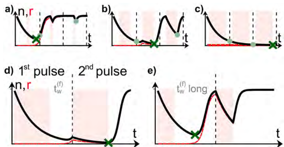
Fig 4. a-c) For a sequence of three pulses, the global population minimum can occur during any of the pulses, depending on the pulse parameters (a: t_r = 6, s = 0 , b: t_r = 30, s = 0 , c: t_r = 45, s = -0.2 ; \tau = 60 for all). The local minimum (within one pulse) is marked with a light green dot, the global minimum is marked with a green cross. In a, the value of n at the minima (green dots) increases successively, such that global minimum occurs during the first pulse. This is because \tau - t_r is large. For b and c, \tau - t_r decreases, implying that the global minimum shifts into the second and third pulse, respectively. Panels d-e show that for s = -1 , the minimum is attained in the second pulse (d), unless t_w^{(f)} is so long that the population can regrow to n = r_{low}^* (e).
