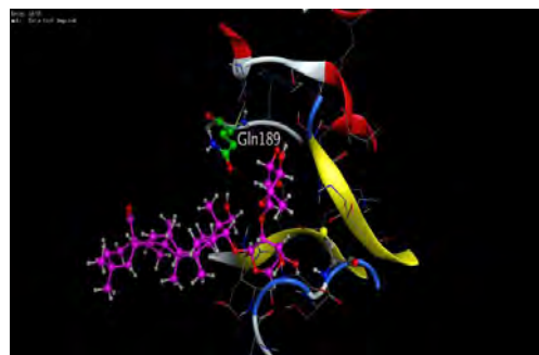
Figure 4A: 3D diagram interaction between \alpha -hederin and 2GTB
