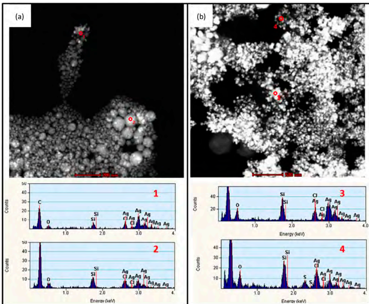
Figure 3. (a,b) HAADF-STEM-EDX characterization of the precipitates formed after the incubation of 17.0 \mu\text{g/mL} \text{AgNO}_3 (equal to an Ag concentration of 10 \mu\text{g/mL} ) in (a) RPMI-1640 and (b) DCCM-1 cell culture medium, at 37 ^\circ\text{C} for 0.5 h. The corresponding STEM-EDX spectra 1–4 were collected from the areas 1–4 marked in (a,b); The precipitates were collected by filtering the solution through 2 kDa filter membrane and were washed three times with DI-water. In both cell culture media, the particles have sizes that range from \sim 20 to \sim 200 nm. STEM-EDX analysis reveals that the precipitates in RPMI-1640 are probably a mixture of silver oxide and silver chloride. The insoluble compounds formed in DCCM-1 likely also contain silver sulphide; (c) Inductively coupled plasma optical emission spectroscopy (ICP-OES) analysis of solubilized silver concentrations of 17 \mu\text{g/mL} \text{AgNO}_3 (equal to an Ag concentration of 10 \mu\text{g/mL} ) in deionized (DI) water, RPMI-1640, DMEM, and DCCM-1 solutions, incubated at 37 ^\circ\text{C} for 0.5 h ( n = 3 ). Although 100% of the free \text{Ag}^+ ions were detected in the \text{AgNO}_3 DI-water solution, the amount of solubilized silver in cell culture media was less than 0.5 \mu\text{g/mL} after incubation. The dissolved \text{Ag}^+ ions are probably sequestered as insoluble precipitates in the cell media, indicating the limitation of using ICP-OES to study the kinetics of \text{Ag}^+ dissolution in cell culture media. Adapted with permission from [143]. Copyright 2013 American Chemical Society.
